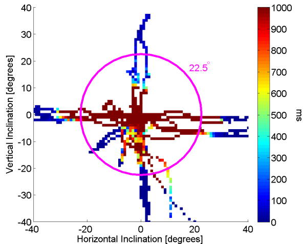
Fig. 6. Reception in the center of the pool with the receiver pointed towards the ceiling. The x-axis corresponds to inclination of the receiver along the short side of the pool. Negative values indicate the receiver pointing towards the left side of the pool and positive values towards the right side. The y-axis corresponds to inclination of the receiver along the long side of the pool. Negative values indicate the receiver pointing towards the transmitter and positive values away from the transmitter (which is located towards the lower right). The origin corresponds to the receiver pointing straight up at the ceiling.
